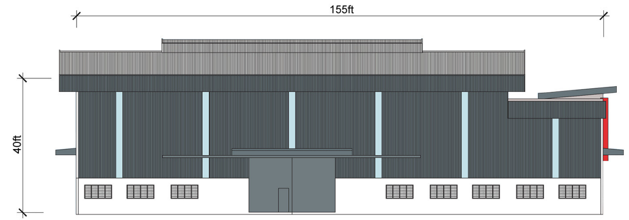
LEFT ELEVATION
