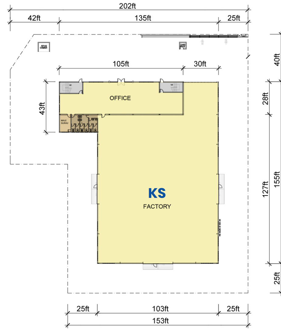
GROUND FLOOR
