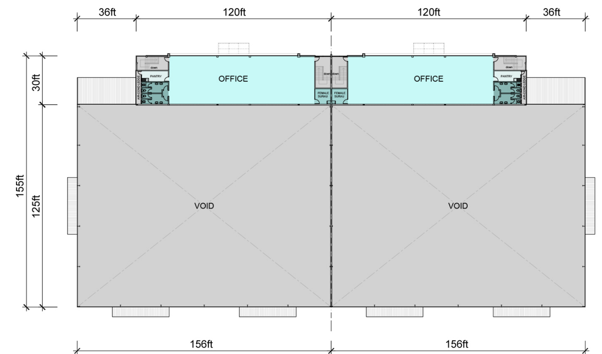
FIRST FLOOR
