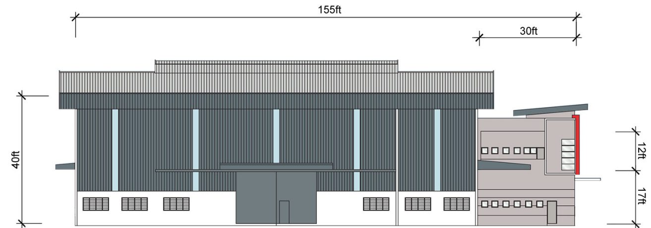
SIDE ELEVATION
