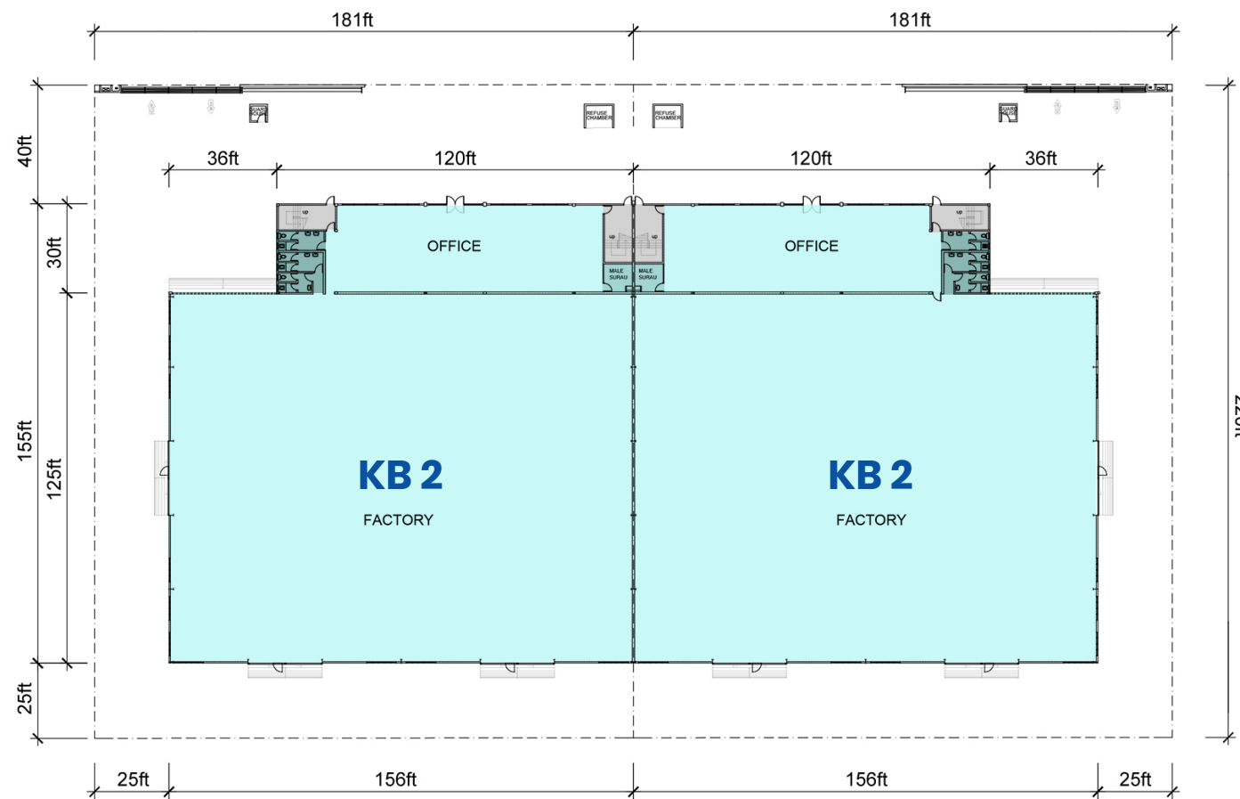
GROUND FLOOR
