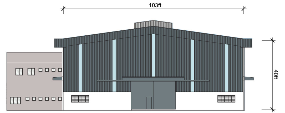
BACK ELEVATION
